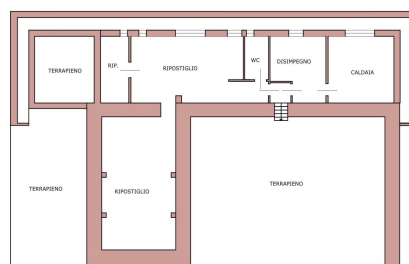
Piano Seminterrato H 2.50 m
