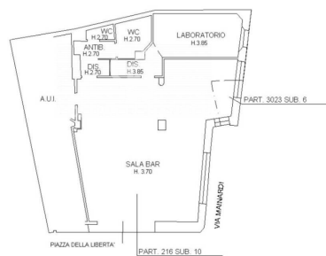
PIANO TERRA
