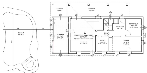
PIANO TERRA scala 1:100
